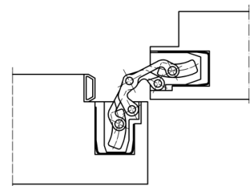
Blockzarge 90°
